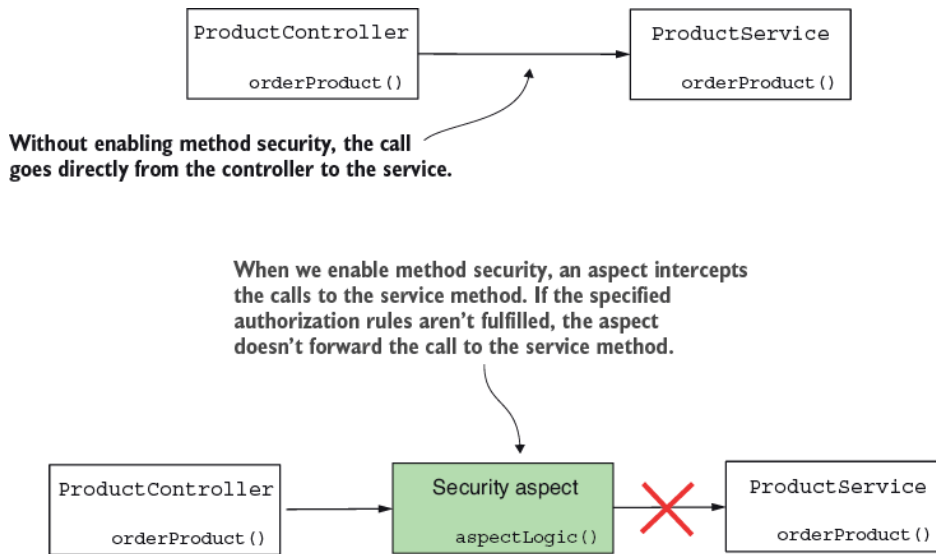
Figure 11.2 When we enable global method security, an aspect intercepts the call to the protected method. If the given authorization rules aren't respected, the aspect doesn't delegate the call to the protected method.
