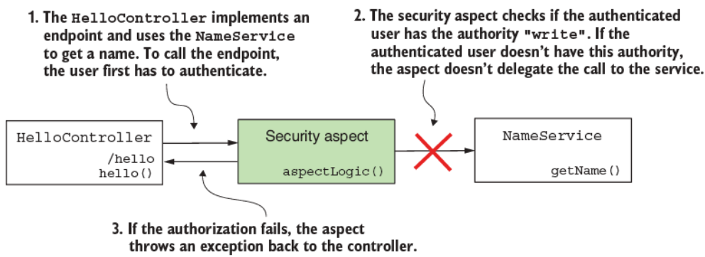
Figure 11.5 To call the getName() method of NameService , the authenticated user needs to have write authority. If the user doesn't have this authority, the framework won't allow the call and will throw an exception.
