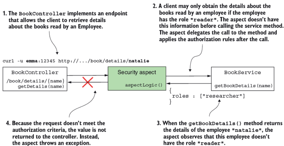
Figure 11.7 With postauthorization, we don't protect the method from being called, but we protect the returned value from being exposed if the defined authorization rules aren't respected.
